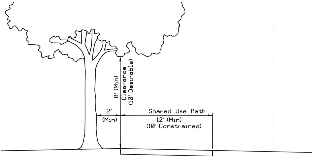
Clearance Detail
